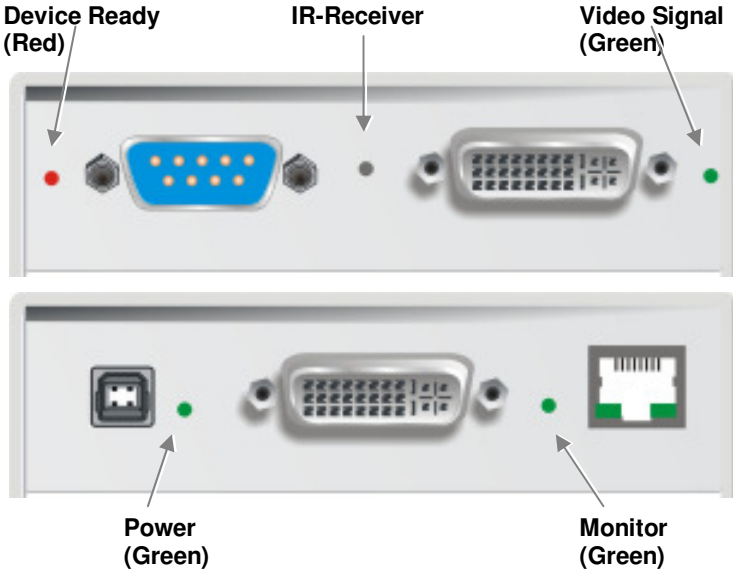
Figure 5 Diagnostic LEDs on RGB to DVI(/VGA) Converter
